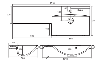
Single tap hole with overflow. Cast Basin. 1010w x 380d x 40h mm
