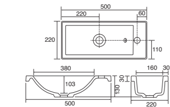
Single tap hole with overflow. Cast Basin. Reversible left/right basin positioning. 500w x 220d x 30h mm
