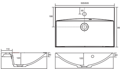
Single tap hole with overflow. Cast Basin. 505w x 380d x 40h mm 605w x 460d x 40h mm
