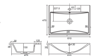
Single tap hole with overflow. Ceramic Basin. 610w x 470d x 35h mm
