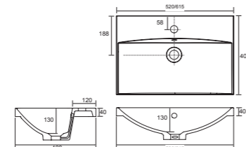
Single tap hole with overflow. 520/615w x 400d x 40h mm
