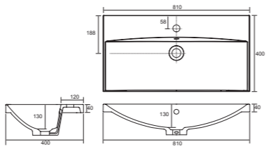
Single tap hole with overflow. 810w x 400d x 40h mm
